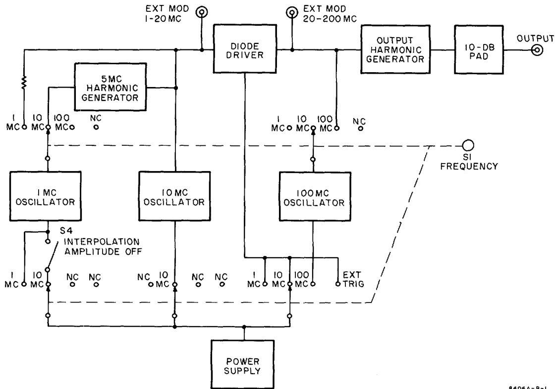
Figure 4-1. Block Diagram
